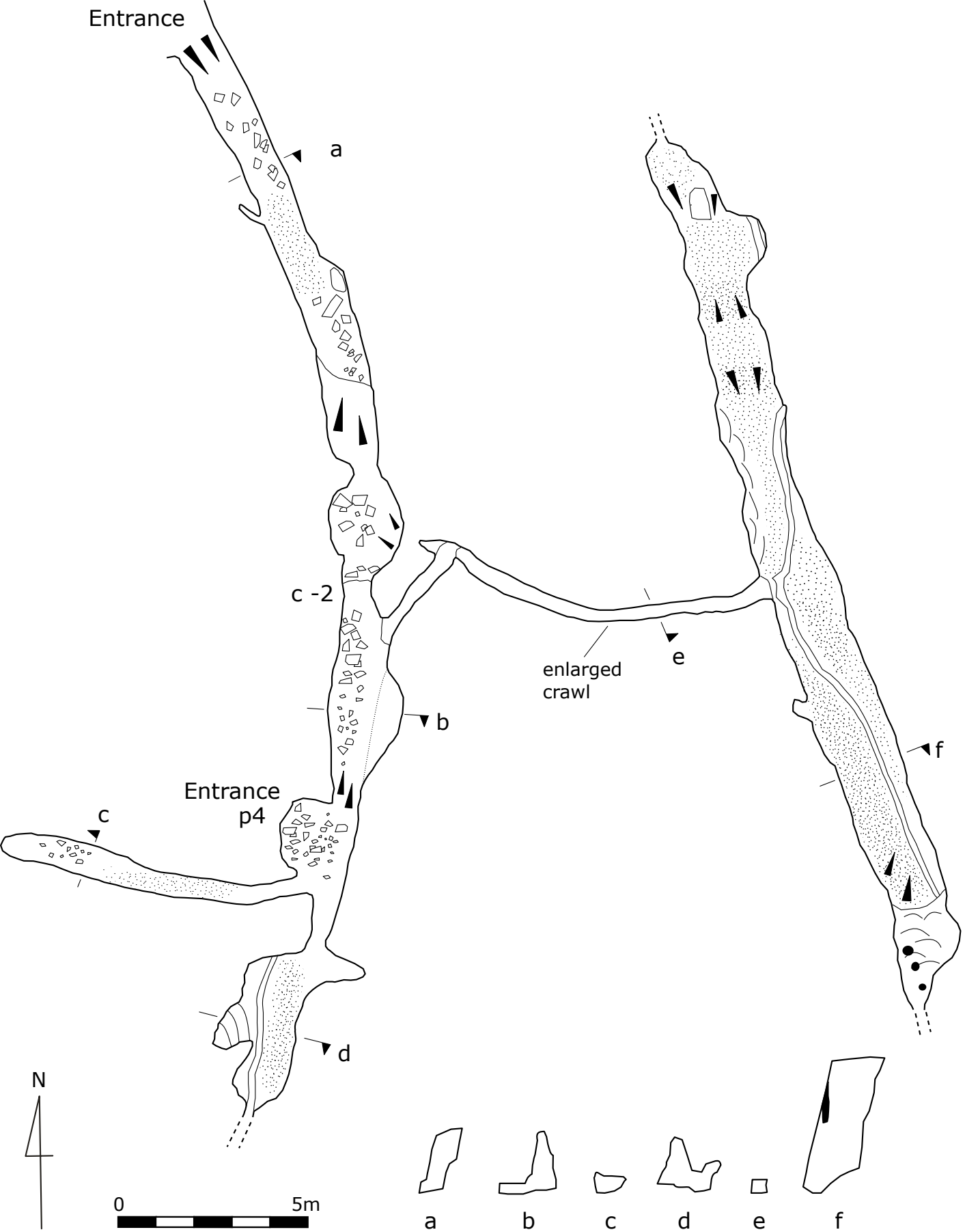
Cueva 1265 Carrales, Matienzo 453458 4795081 256m Length 80m Surveied Sep. 2020 PS
